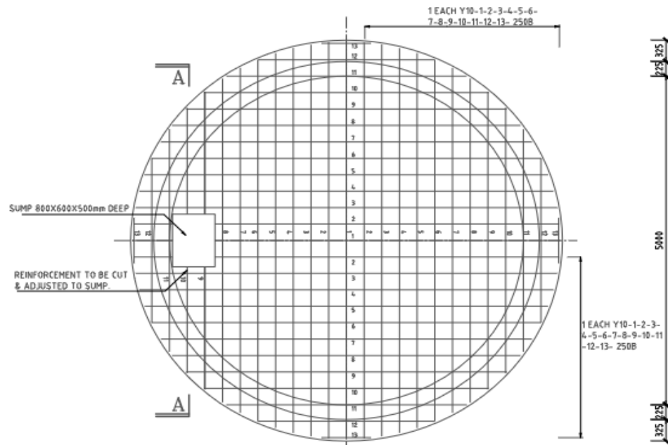
BOTTOM REINFORCEMENT OF FLOOR SLAB SCALE 1:50
