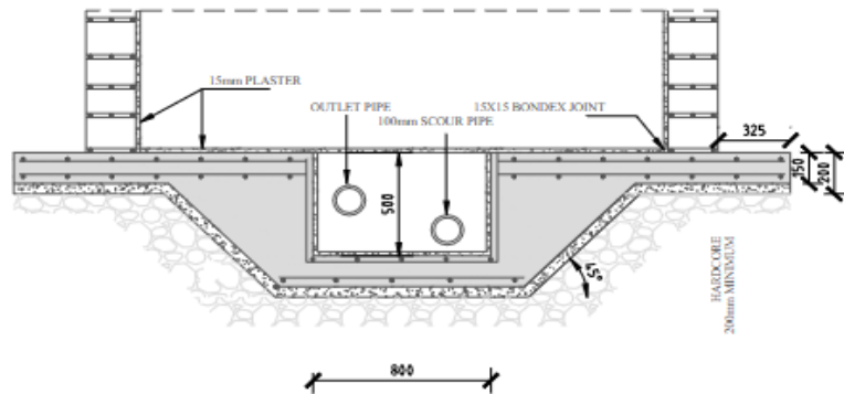
BOTTOM REINFORCEMENT OF FLOOR SLAB SCALE 1:50
