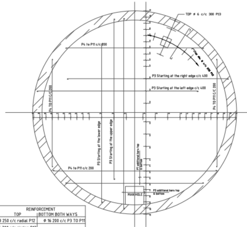
ROOF REINFORCEMENT SCALE 1:50
