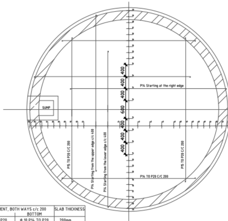
FLOOR REINFORCEMENT SCALE 1:50
